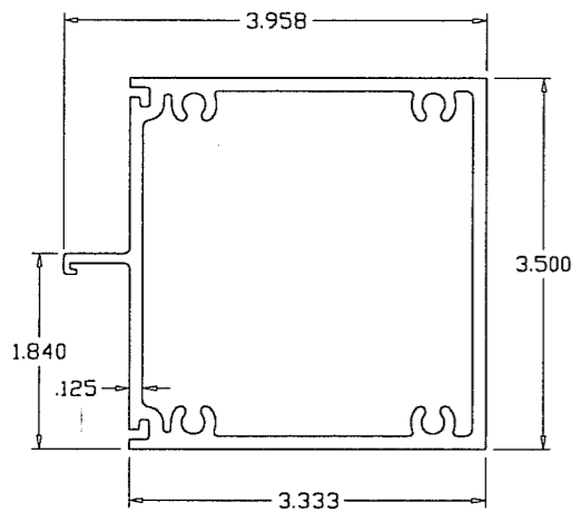
⑥ FRAME HORIZONTAL
