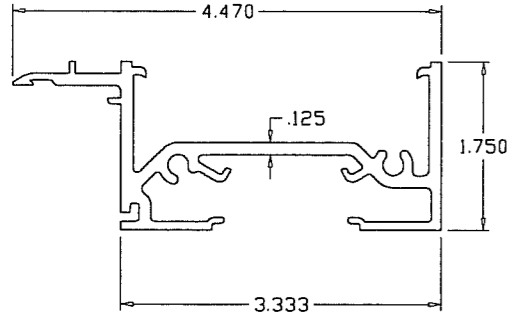
② FRAME HEAD/SILL
