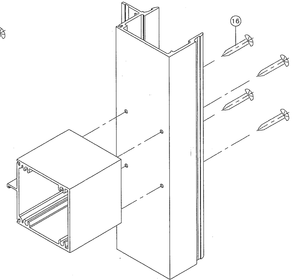
FRAME HORIZONTAL CORNER
