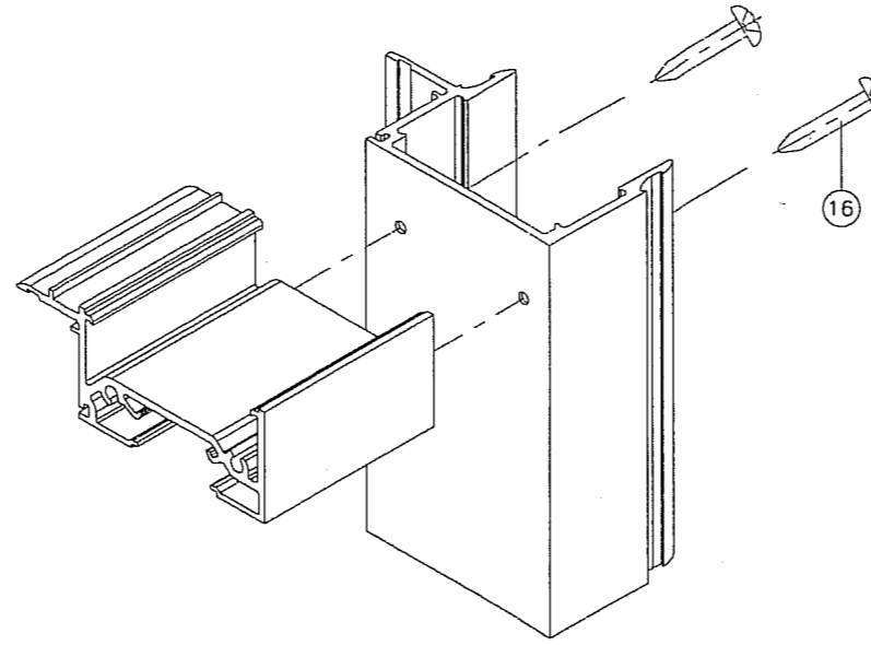
FRAME TOP/BOTTOM CORNER
