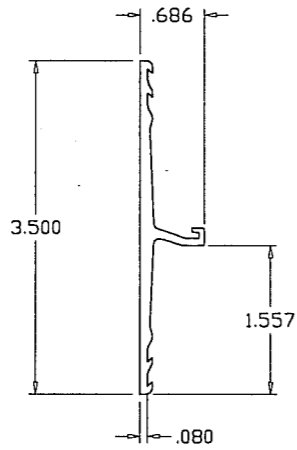
④ GLAZING RETAINER (HORIZONTAL)
