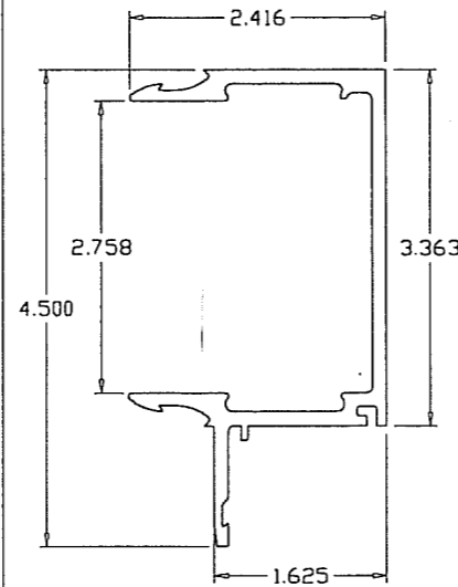
⑧ MALE MULLION
