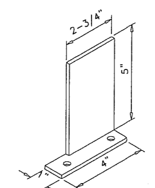
DOOR MULLION INSTALLATION CLIP 1 X 5 X 3/16" ALUM ANGLE
