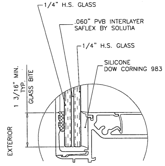
GLAZING DETAIL
